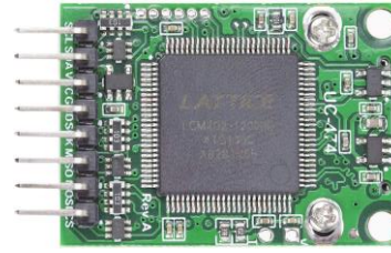
Figure 69 ArduCAM Back. Permission to reproduce requested.
