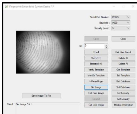
Figure 95 Picture of fingerprint on demo software. Permission to reproduce requested.
