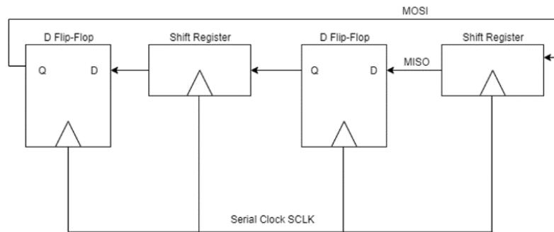
Figure 8 SPI Diagram
