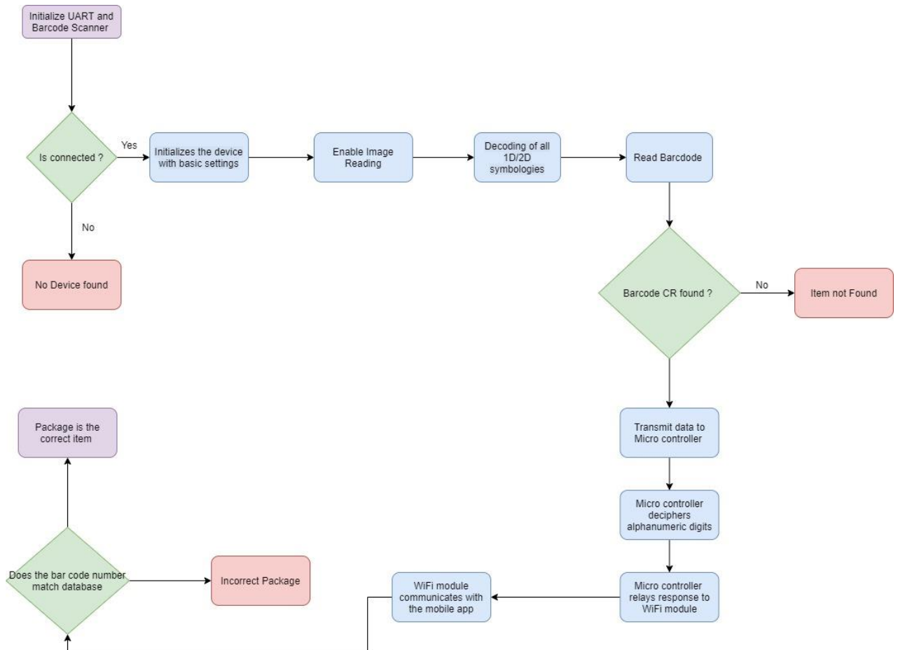
Figure 80 Barcode Scanner Software Flowchart
