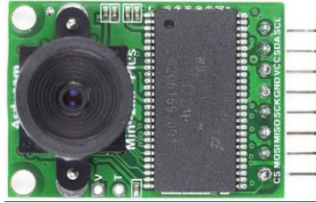
Figure 68 ArduCAM Front. Permission to reproduce requested.
