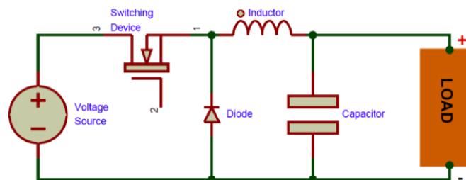
Figure 49 Buck Converter
