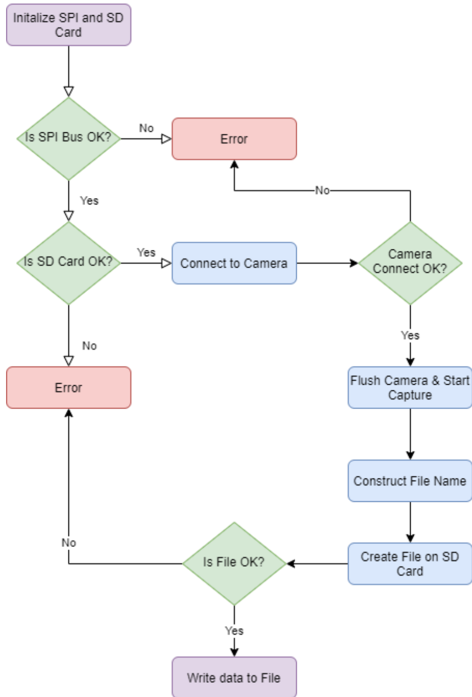
Figure 82 General camera capture software logic
