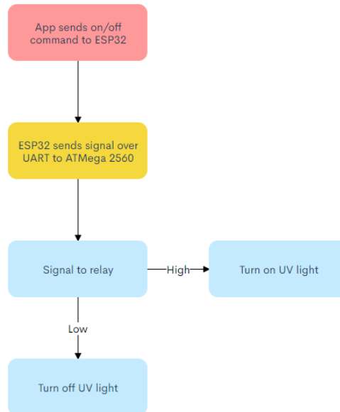
Figure 76 UV light flowchart
