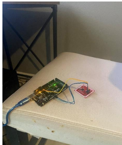
Figure 101 Arduino connected with the RFID module.
