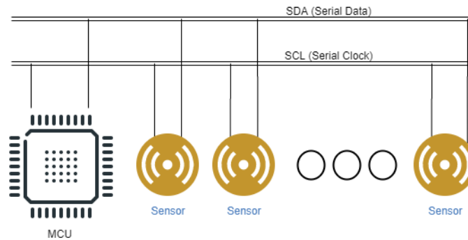
Figure 7 I2C Diagram
