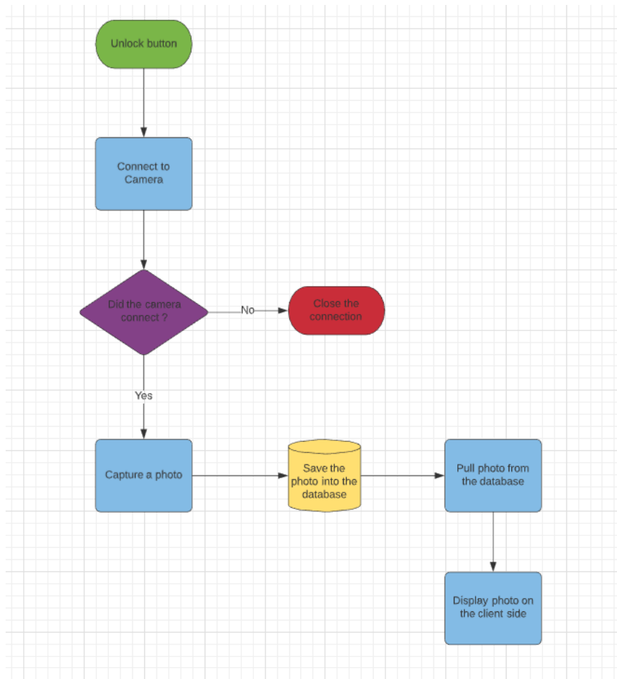
Figure 86 View Pictures Software Logic Flowchart
