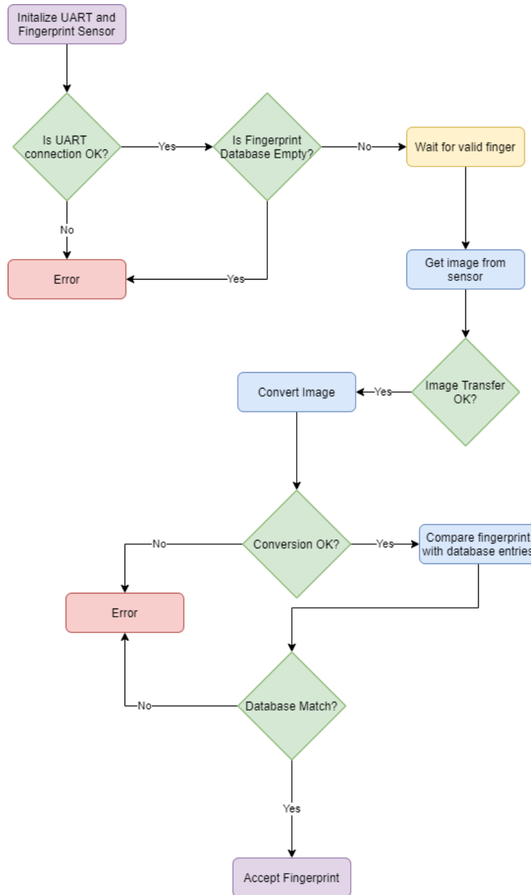
Figure 81 General fingerprint scan software logic
