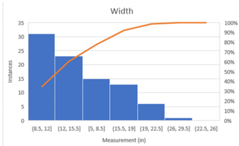
Figure 14 Width
