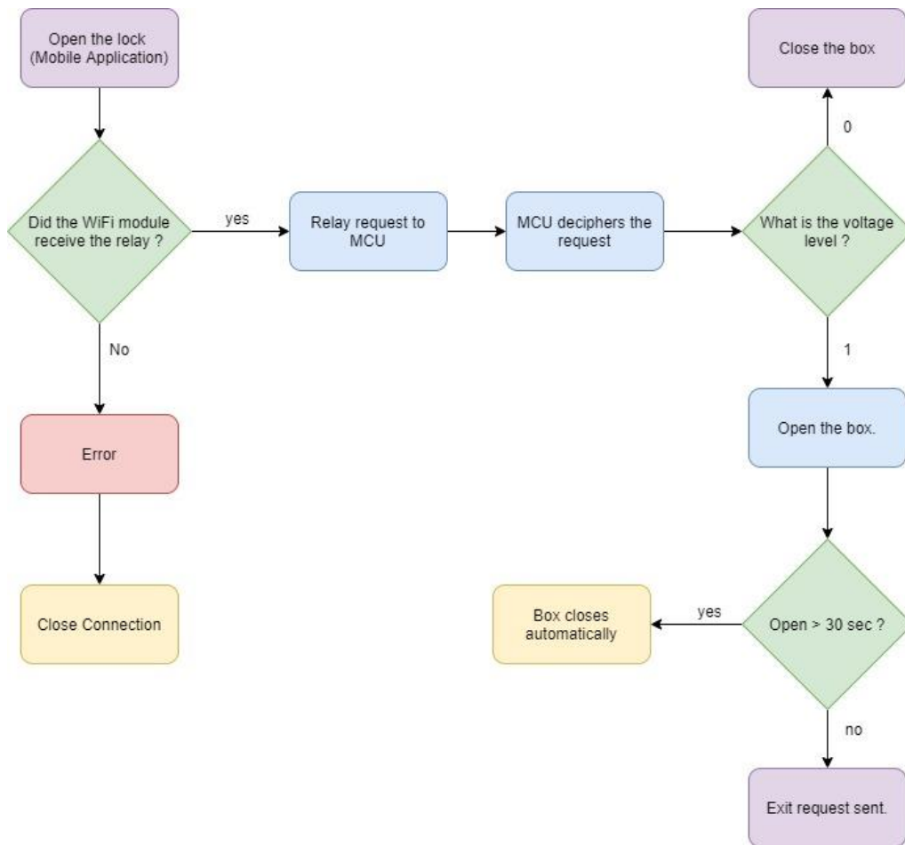
Figure 79 General power lock software logic
