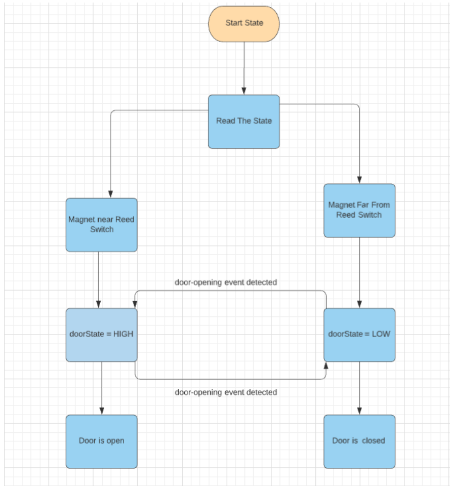
Figure 78 Open/Close Sensor Software Flowchart
