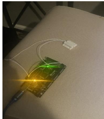
Figure 105 The Arduino with the reed switch in a closed state.
