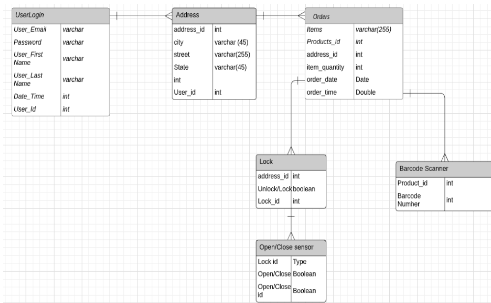
Figure 83 Our Database design and layout
