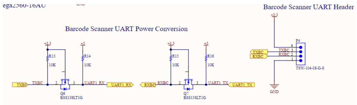
Figure 61 Barcode Scanner Header
