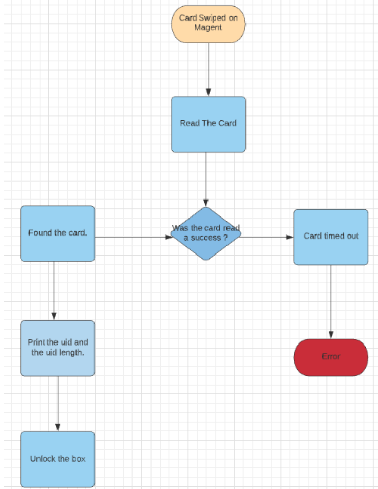
Figure 77 NFC/RFID Software Flowchart
