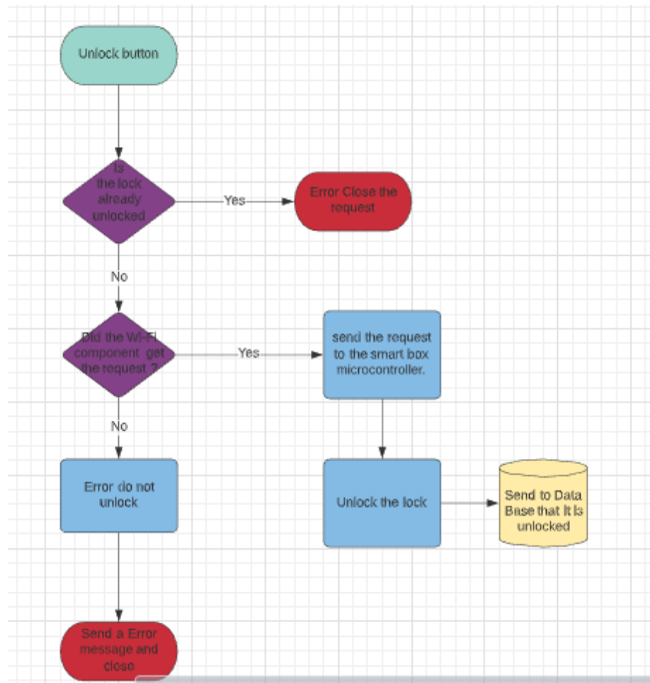
Figure 85 Unlock Button Software Logic Flowchart
