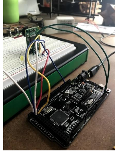
Figure 100 ArduCAM test picture and hardware wiring
