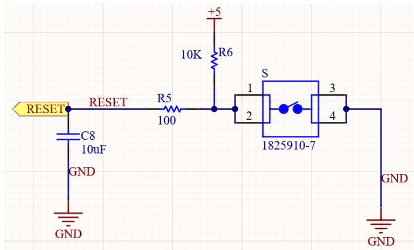
Figure 73 Reset button schematic with debouncing
