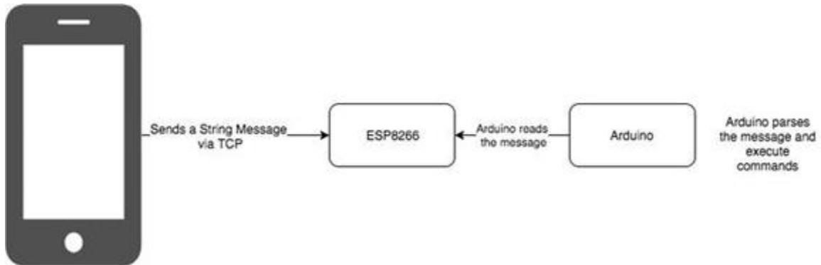
Figure 24 Protocol Schematic
