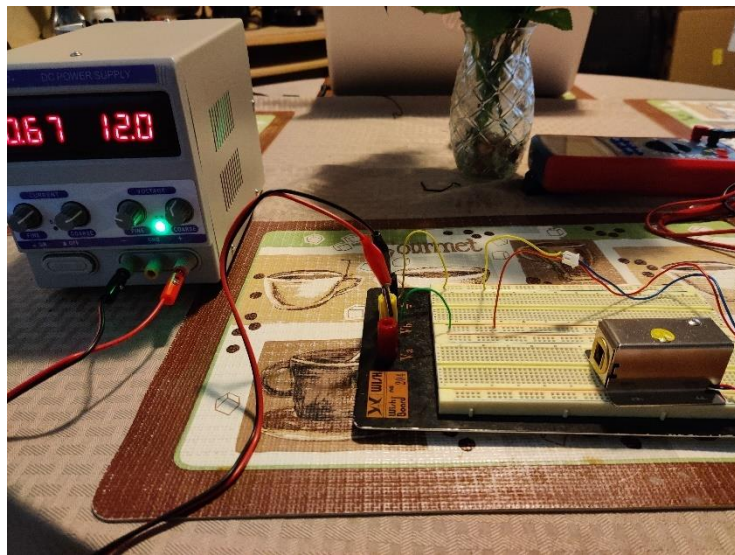
Figure 93 Barcode Scanner in Unlock Position (12V)
