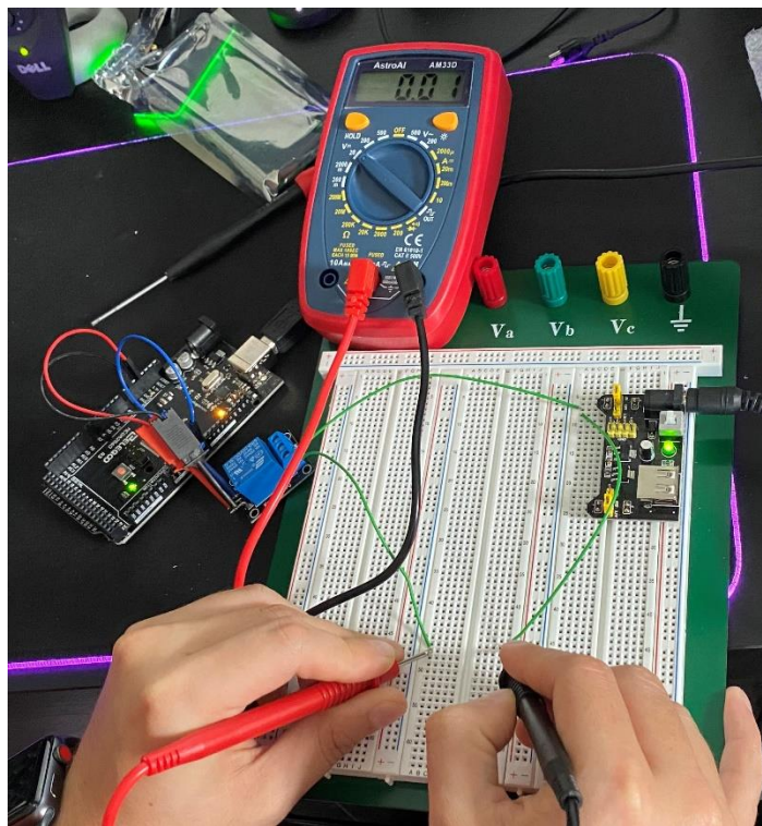
Figure 87 Relay testing off
